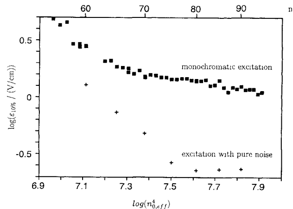
FIG. 3. Ionization threshold fields \epsilon_{10\%} in laboratory units as a function of the initial principal quantum number n_0 for coherent signal excitation \epsilon_{c,10\%} and for broadband noise excitation \epsilon_{N,10\%} . Interaction time \tau = 5 \mu\text{s} .
