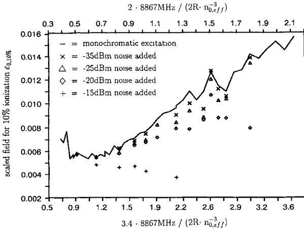
FIG. 1. Normalized threshold field for 10% ionization, \varepsilon_{0,10\%} , as a function of the normalized frequency. \varepsilon_{0,10\%} = \varepsilon_c(10\%) \times n_{0,\text{eff}}^4 , n_{0,\text{eff}} = n_0 - \delta , where \delta = 2.64 is the quantum defect of the initial p state [4]. Two different transitions have been used to normalize the frequency: \omega_{ps} = 2 \times 8867 \text{ MHz} / 2Rn_{0,\text{eff}}^{-3} for the transition np \rightarrow (n+1)s (upper scale) and alternatively \omega_{pd} = (3.4 \times 8867 \text{ MHz}) / 2Rn_{0,\text{eff}}^{-3} for the transition np \rightarrow (n-1)d (lower scale). R denotes the Rydberg constant in MHz. The solid line connects the values measured for monochromatic excitation. The points represent threshold fields observed in the presence of additive noise. We used four different levels of integrated noise power: \times , -35 dBm; \Delta , -25 dBm; \diamond , -20 dBm; and + , -15 dBm. The statistical and systematic errors of \varepsilon_{0,10\%} are estimated to be 5% each.
