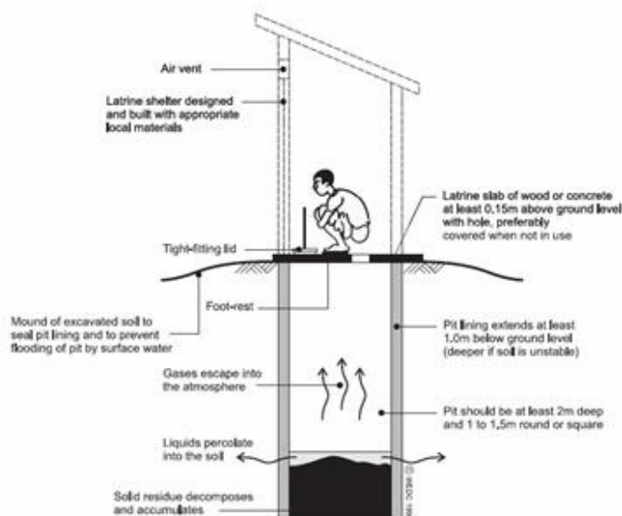
Figure 5: Pit Latrine Source: STAUFFER & SPUHLER 2011
